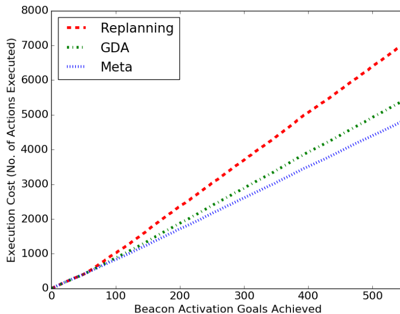
Figure 5. Average execution cost as a function of goal achieved in the NBeacons domain.
