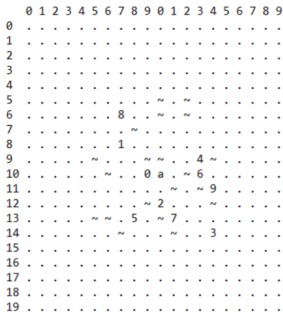
Figure 4. NBeacons Example Scenario. The symbol a represents the agent, integers between 0-9 are the locations of beacons, and ~ represents a sand pit.
