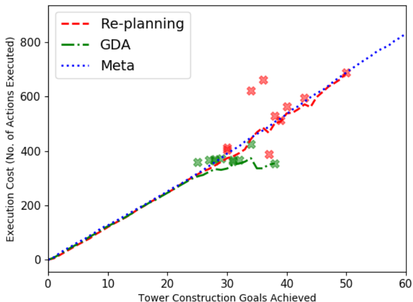
Figure 6. Average execution cost as a function of goals achieved in the Aggressive Arsonist domain. The colored \times 's on the graph indicate the last goal achieved in each run before failing.
