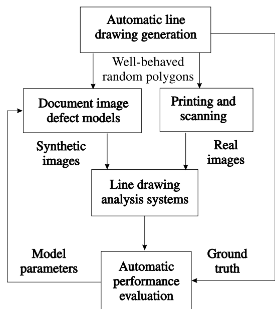
Figure 1: Overview of the paper.
