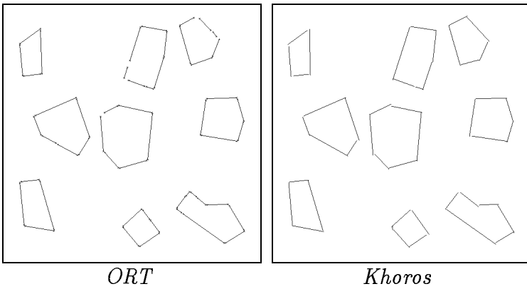
Figure 10: ORT and Khoros results under low noise.
