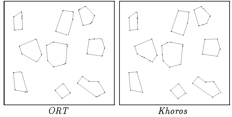
Figure 12: ORT and Khoros results under high noise.
