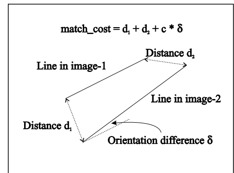
Figure 3: Cost for matching two lines.
