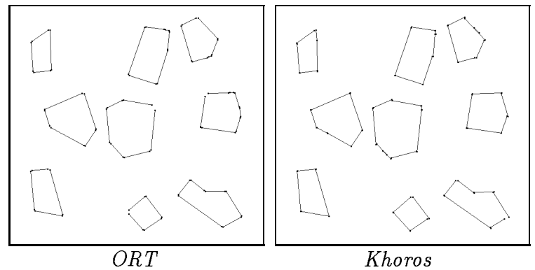
Figure 13: ORT and Khoros results under low noise.
