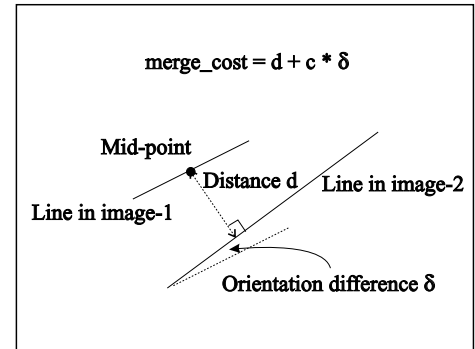
Figure 2: Cost for merging one line into another.
