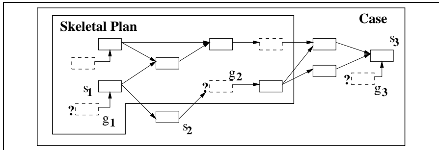
Figure 6: Abstract configurations of an skeletal plan and a case
