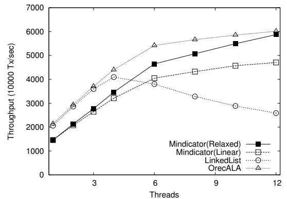
(b) x86
