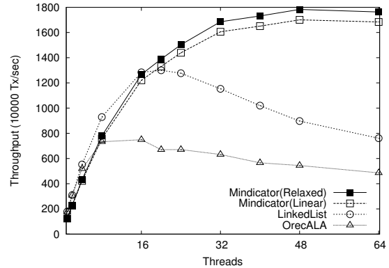
(a) Niagara2
