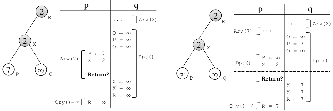
(c) p.Arrive (7) encounters an unfinished q.Depart () at X. Is 2 being removed from X? (d) p.Depart (7) encounters an unfinished q.Depart () at X. Can 7 reappear at X?
