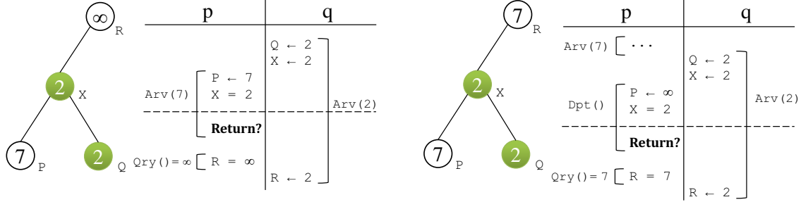
(a) p.Arrive (7) encounters an unfinished q.Arrive (2) at X. Has 2 reached R? (b) p.Depart () encounters an unfinished q.Arrive (2) at X. Has 7 been removed from R?
