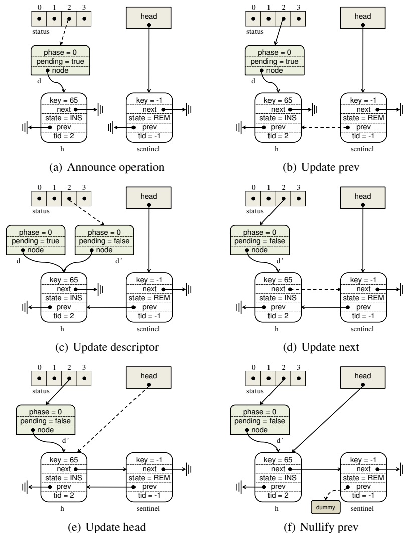
Fig. 3: Wait-free ENLIST Implementation Extended from the Kogan-Petrack Algorithm
